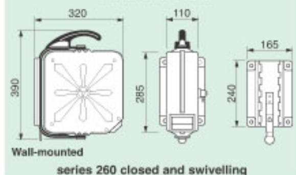
Overall dimensions
